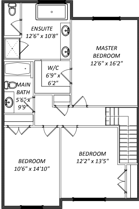
SECOND FLOOR - 968 SQ FT
